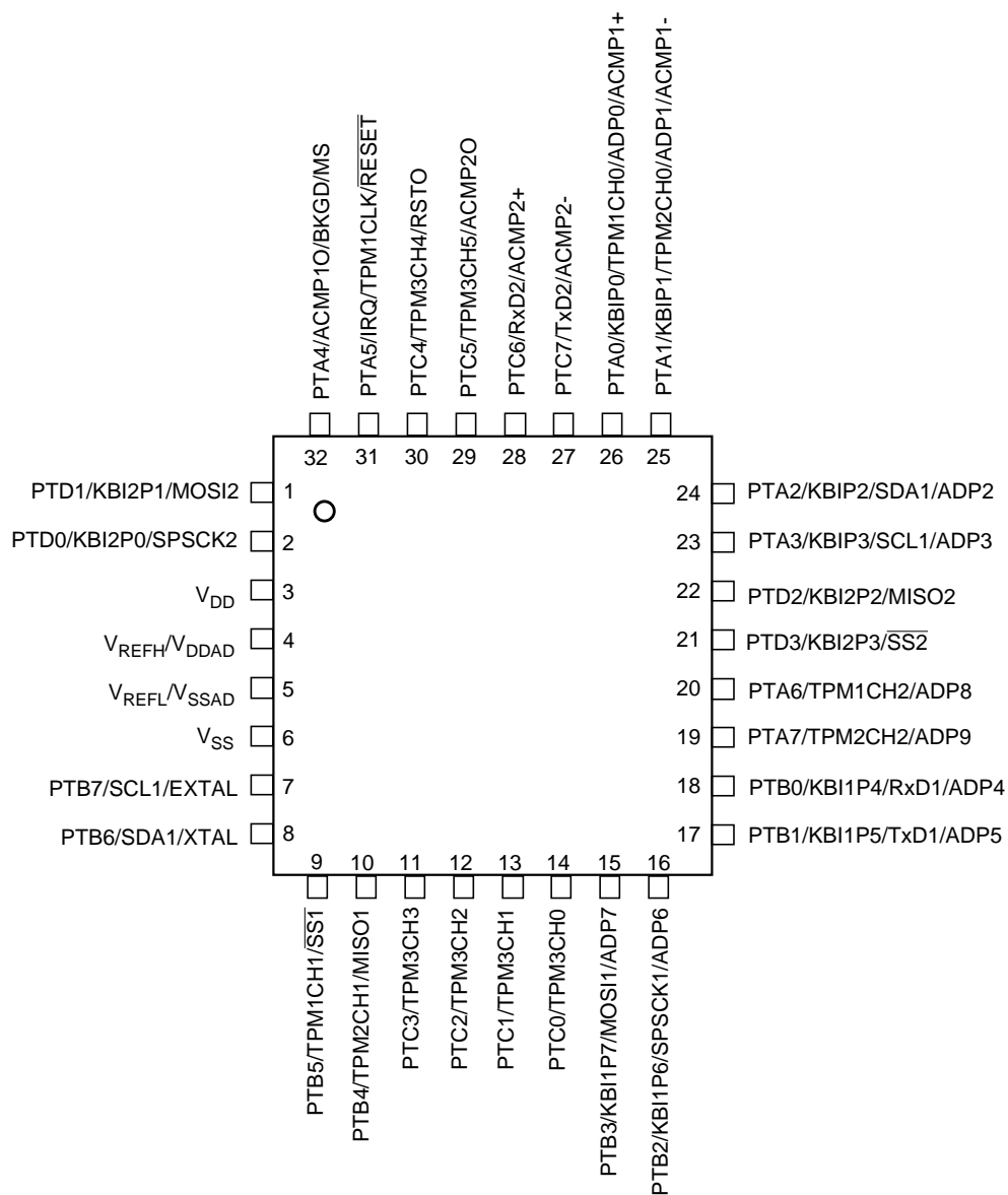
Figure 2-5. 32-Pin LQFP
